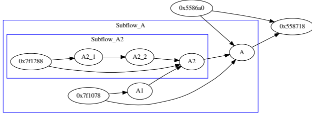
Fig. 5: Visualization of a nested subflow using the dump method.
