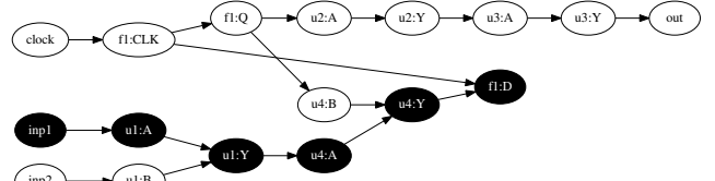
Fig. 8: An example task dependency graph of a single timing update.
