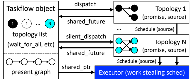
Fig. 3: Program flow of dispatching task dependency graphs.
