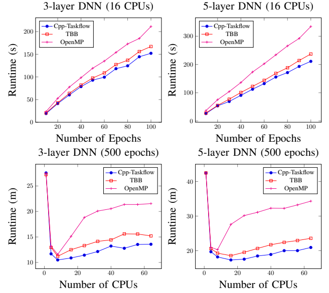
Fig. 12: Performance comparisons between Cpp-Taskflow, TBB, and OpenMP on training two different DNN classifiers.
